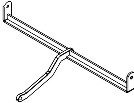
Image 19: CR-LINK / Adapter allows Top (max 6x) - Sub combination without additional frame.
