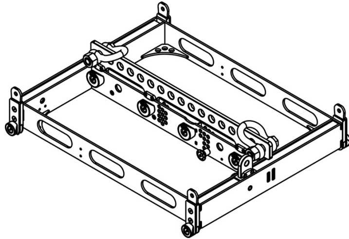
Image 14: FR-AR-Set/ Frame for flying or ground stacking AiRAY/ ViRAY/ CiRAY or SC2-F/ SCV-F in various combinations
