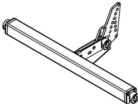
Image 18: CGA/ CIRAY Ground Stack Adapter. Max 8x CIRAY cabinets can be stacked on SC2-F/ SCV-F.
