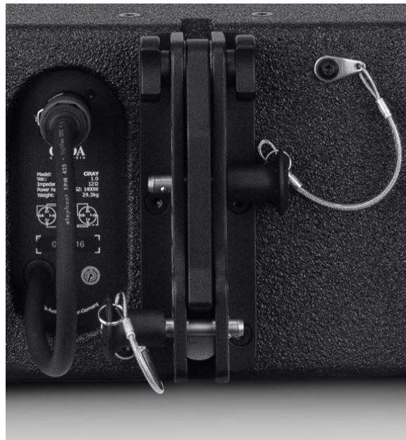
Image 13: Coda-Pin-R ViRAY in single cabinet transport position
