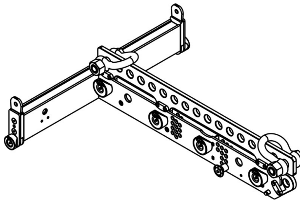
Image 15: FRT-AR Set/ Frame for flying AiRAY/ ViRAY/ CiRAY
